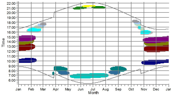
1: NORDEX N117 2400 117.0 IO! hub: 120,0 m (TOT: 178,5 m) (1.1)
